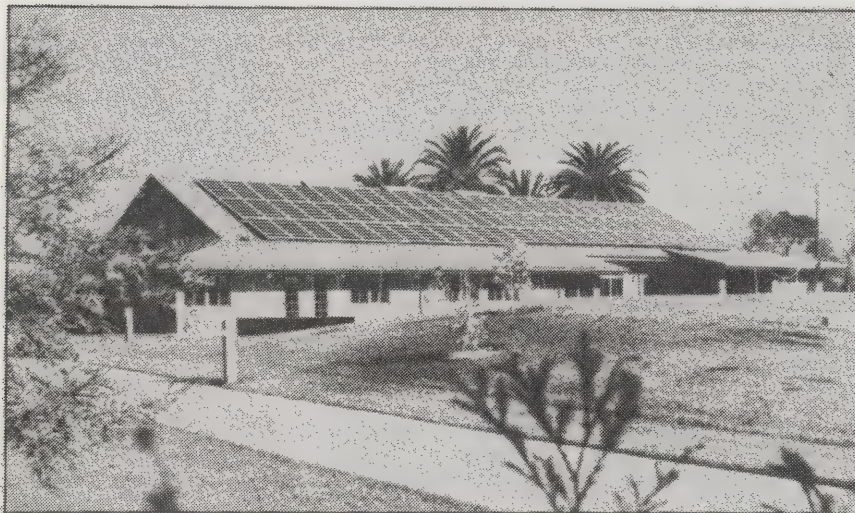
◀ The City of Dixon [California] recently dedicated this 20kW. photovoltaic energy system on top of the roof of their City Hall.
